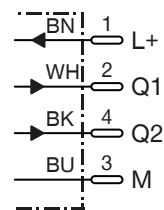
Connection diagram
