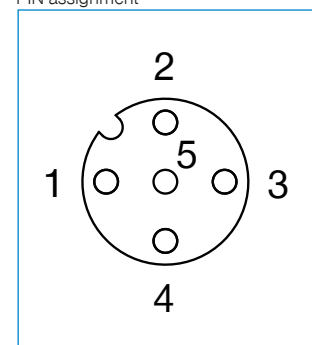
PIN assignment
