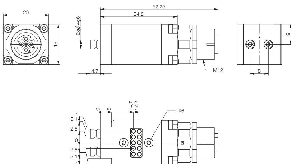
PIN assignment
