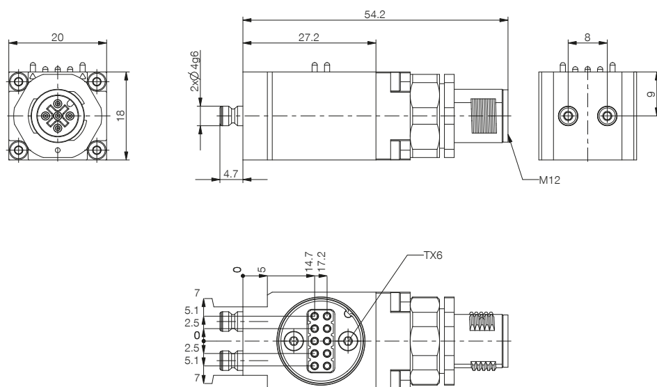
PIN assignment
